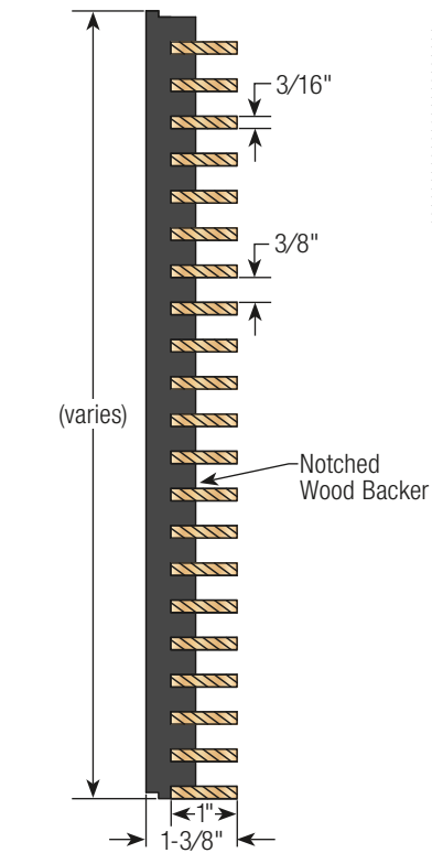
MG1—Side View
