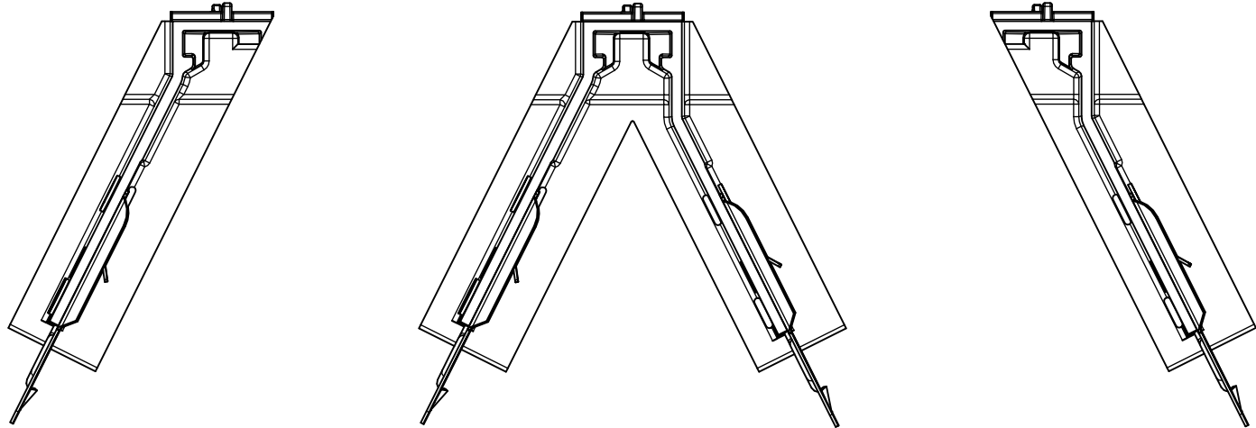
BP75AB60L Suprafine 60° Left Angle Bracket BP75AB60D Suprafine 60° Double Angle Bracket BP75AB60R Suprafine 60° Right Angle Bracket
