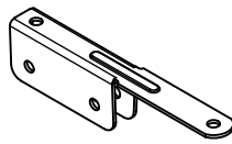
BPPAC Perimeter Angle Clip SCALE 1 / 2
