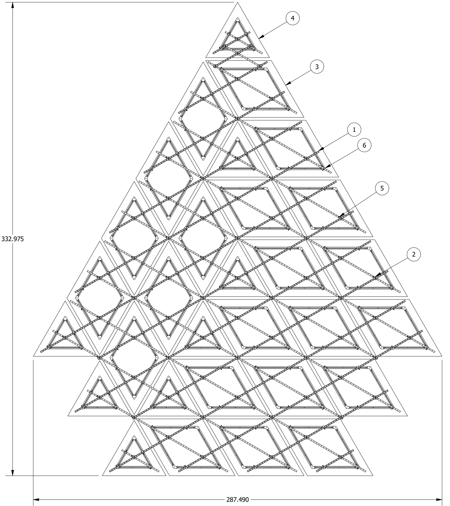
REAR VIEW SCALE 1 / 40
