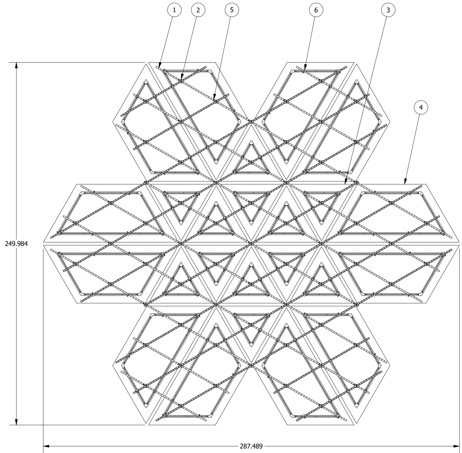
REAR VIEW SCALE 1 / 40
