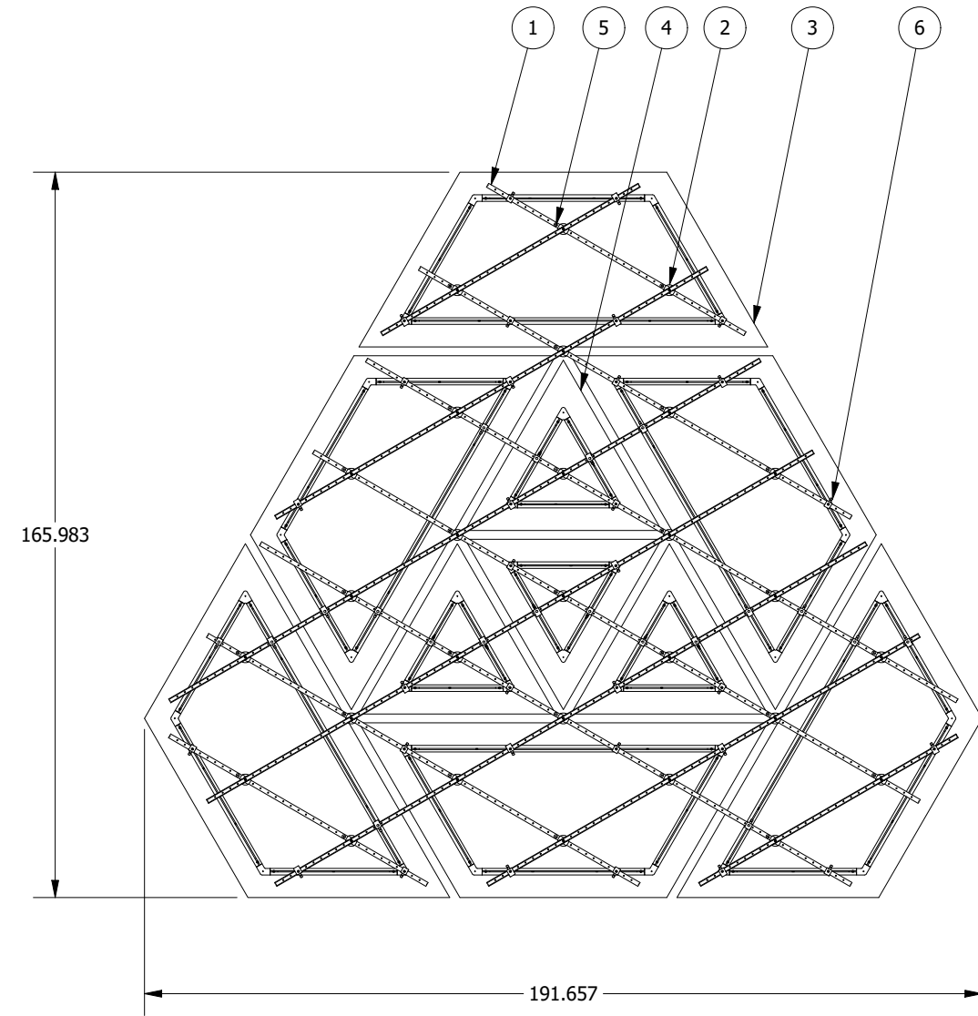
REAR VIEW SCALE 1 / 40
