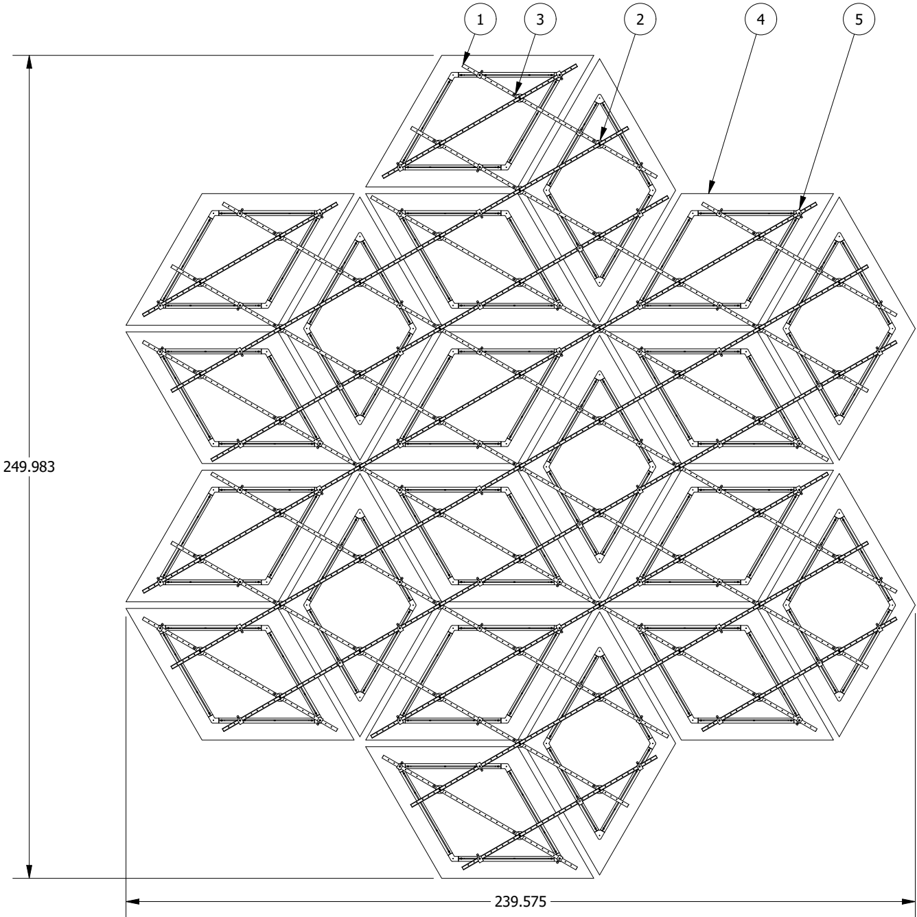
REAR VIEW SCALE 1 / 40
