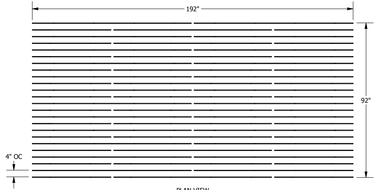
PLAN VIEW
