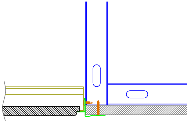
TRADITIONAL FRAMING
