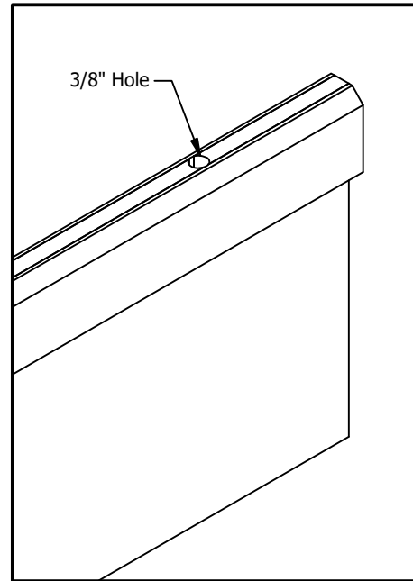
STEP 2 Drill 3/8" hole in top of blade, about 1" deep
