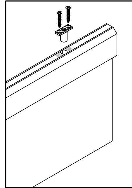
STEP 4 Insert hanging kit into hole & secure with screws
