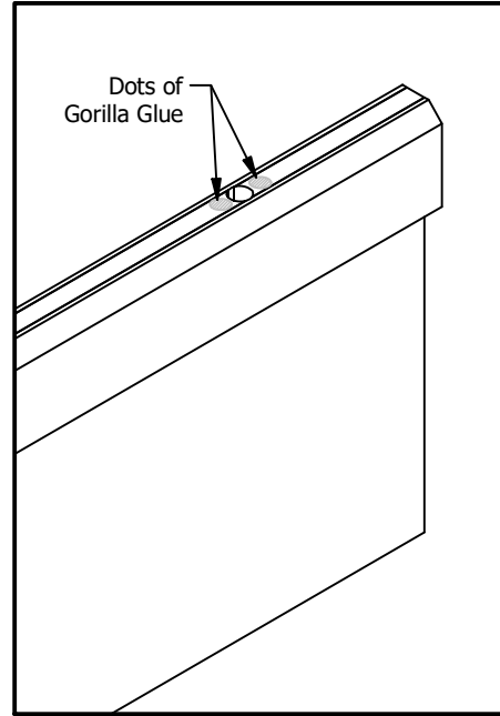
STEP 3 Add dots of gorilla glue to both sides of the hole
