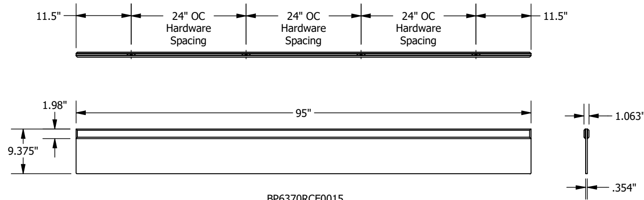
BP6370RCE0015 Reinforced Rectangular Panel - 8' Width, 9.375" Depth
