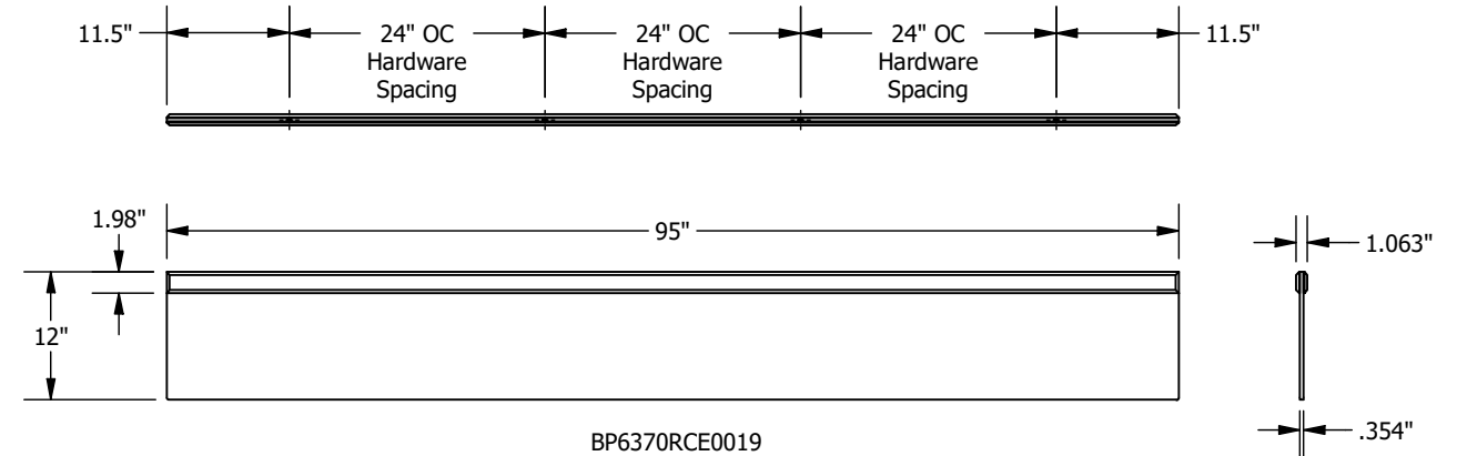
BP6370RCE0019 Reinforced Rectangular Panel - 8' Width, 12" Depth
