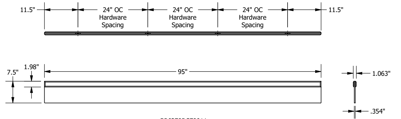
BP6370RCE0011 Reinforced Rectangular Panel - 8' Width, 7.5" Depth
