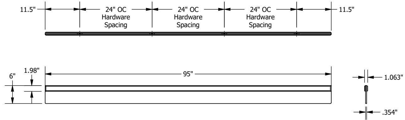
BP6370RCE0001 Reinforced Rectangular Panel - 8' Width, 6" Depth
