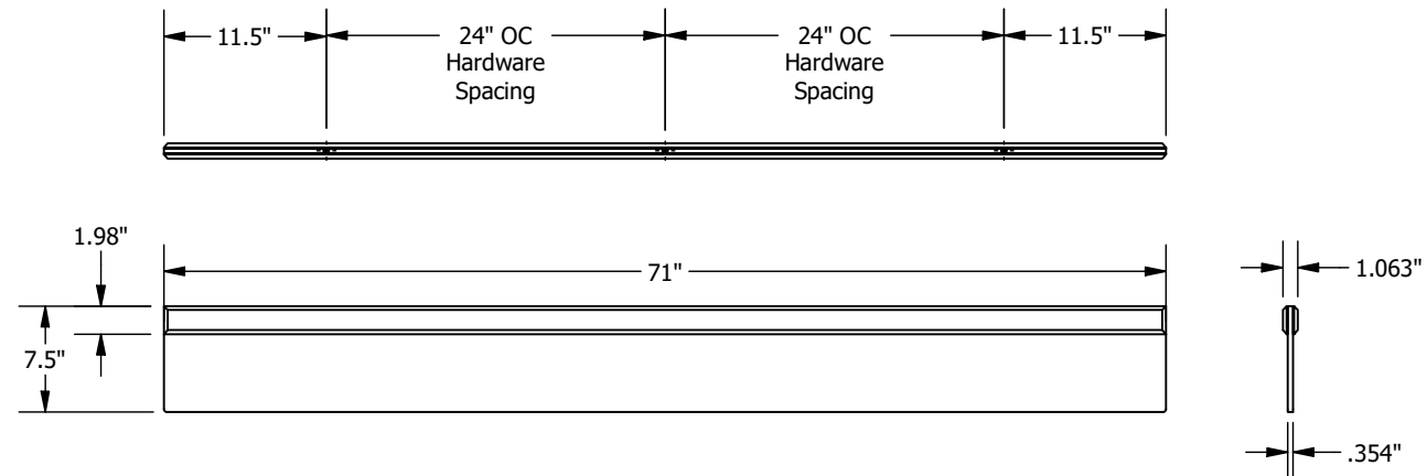
BP6370RCE0010 Reinforced Rectangular Panel - 6' Width, 7.5" Depth
