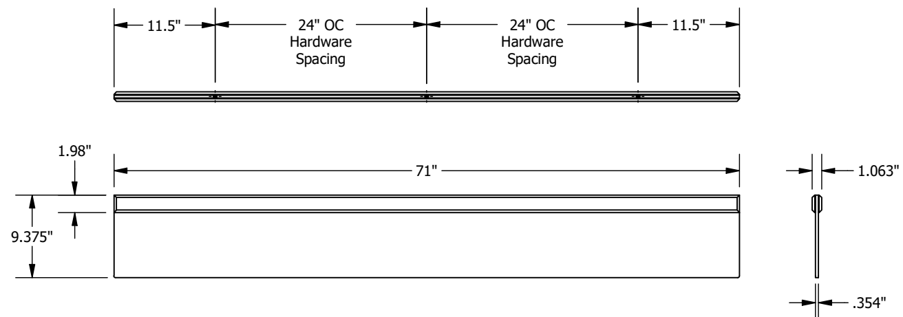
BP6370RCE0014 Reinforced Rectangular Panel - 6' Width, 9.375" Depth
