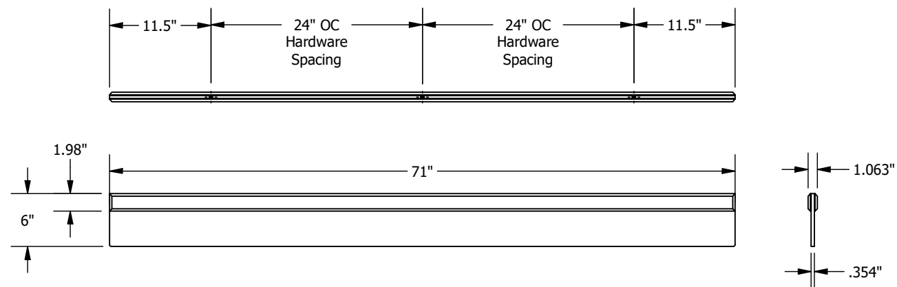
BP6370RCE0007 Reinforced Rectangular Panel - 6' Width, 6" Depth
