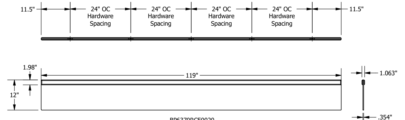
BP6370RCE0020 Reinforced Rectangular Panel - 10' Width, 12" Depth
