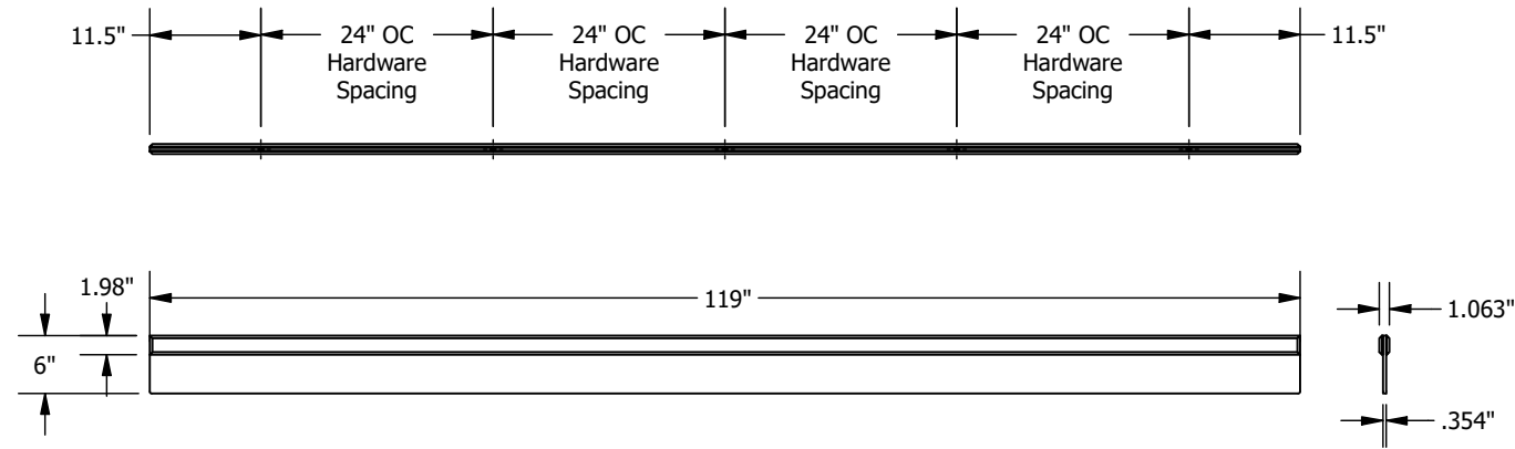
BP6370RCE0008 Reinforced Rectangular Panel - 10' Width, 6" Depth
