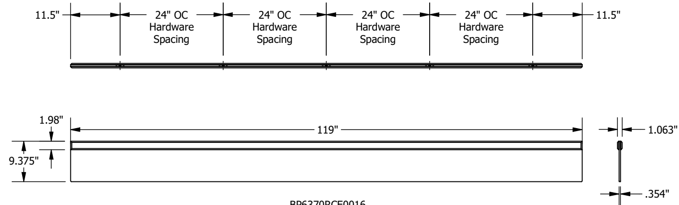
BP6370RCE0016 Reinforced Rectangular Panel - 10' Width, 9.375" Depth
