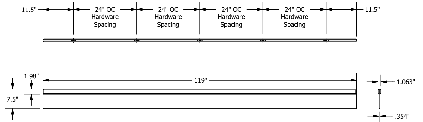
BP6370RCE0010 Reinforced Rectangular Panel - 10' Width, 7.5" Depth
