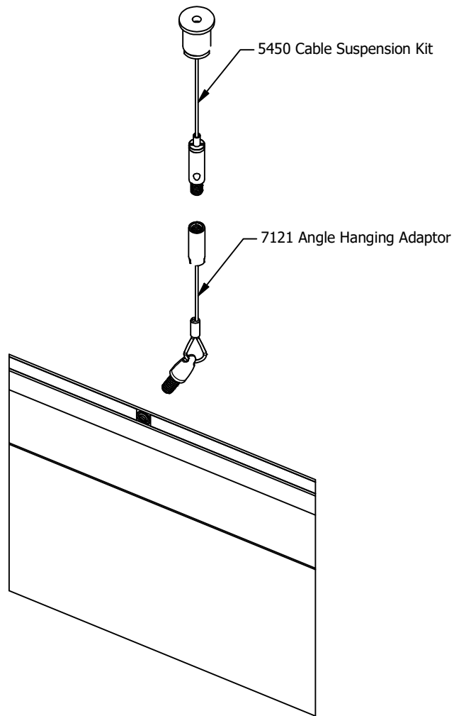
5450 Cable Suspension Kit and 7121 Angled Hanging Adaptor Installed Exploded View
