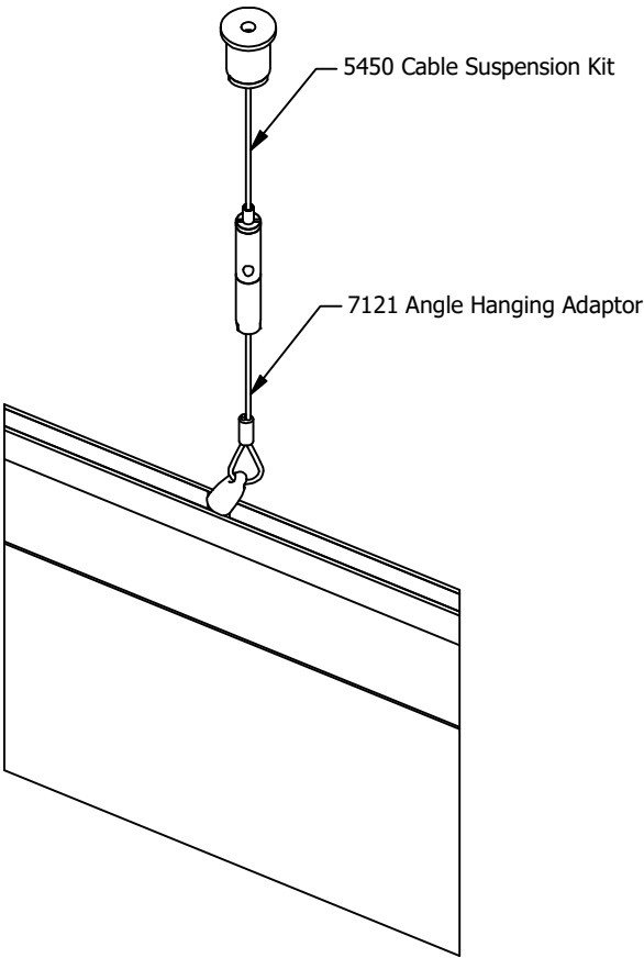
5450 Cable Suspension Kit and 7121 Angled Hanging Adaptor Installed View
