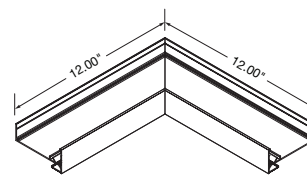
Classic Ceiling-to-Wall Inside Corner
