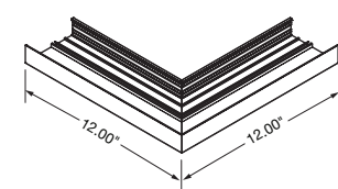
Classic Ceiling-to-Ceiling Inside Corner
