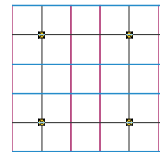
30" x 30" Ceiling layout with lights 7-1/2' apart
