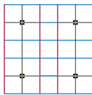
2' x 2' Ceiling layout with lights 6' apart
