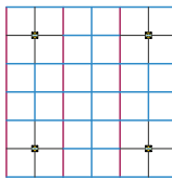
2' x 2' Ceiling layout with lights 8' apart
