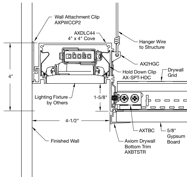
4" x 4" Direct Light Cove – AXDLC44
