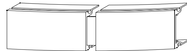
Insert splice plate in joint and close to about 1/2"
