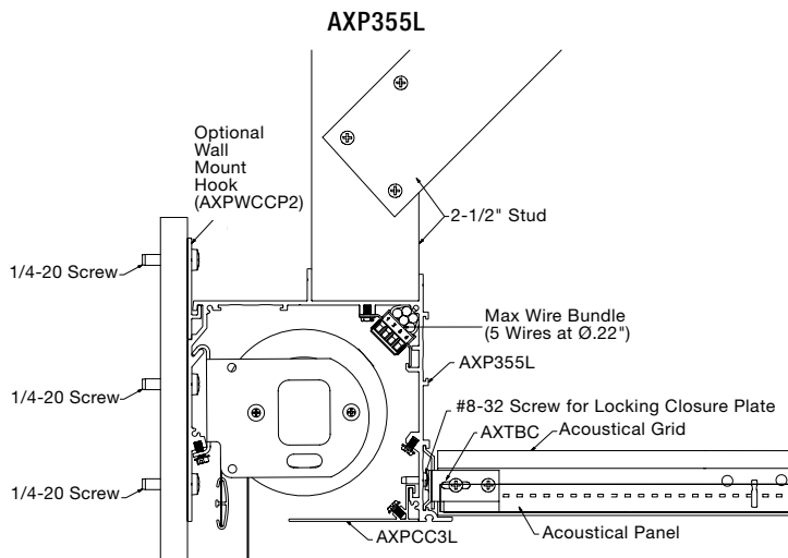
Motorized Shade Pocket – For Attachment with 2-1/2" Studs
