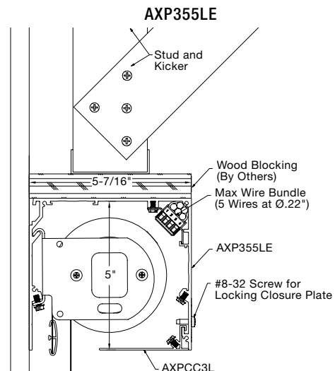
Motorized Shade Pocket – For Traditional Framing
