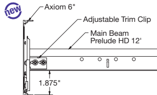
Axiom® Vector® Trim
