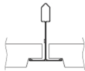
Angled Tegular 斜角跌级 (D7396, D7397)
