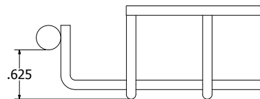
Edge Detail for Welded Tegular
