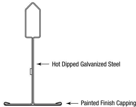
Figure 1. Composition of Interlude® XL® Suspension Systems
