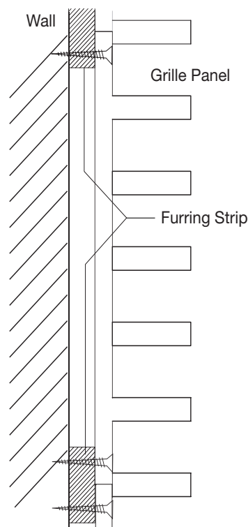
Grille Panel Backer
