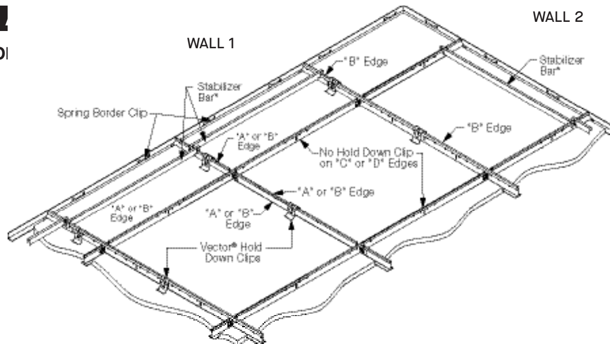
Vector® Hold-down Clip (Item #442B)
