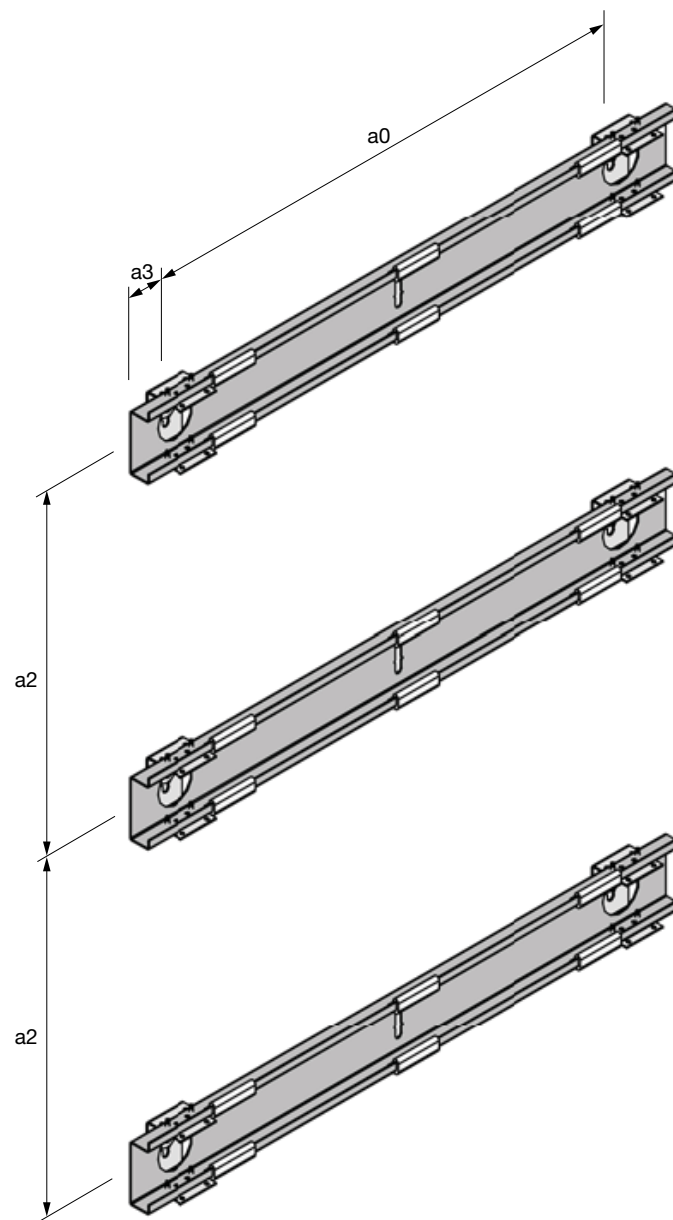
Detail of fixing point with wall anchor
