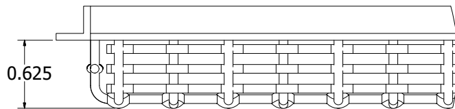
Edge Detail for Woven Tegular
