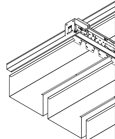
Unattached wall, screw through BERC2 slot
