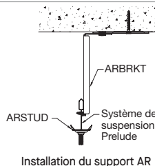
Installation du support AR
