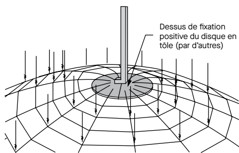
Renfort vertical
