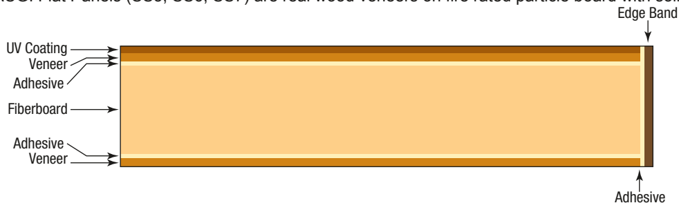
Figure 1. Composition of a WoodWorks® ACGI Ceiling Panel
