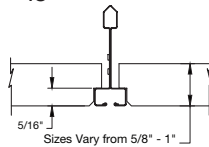
Beveled Tegular for 9/16" SILHOUETTE® 1/8" Reveal Molding F
