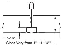
Square Tegular for 9/16" SILHOUETTE® 1/8" Reveal Molding F
