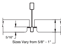
Beveled Tegular for 9/16" INTERLUDE® Molding F
