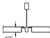
METALWORKS 5/16" Square Tegular for INTERLUDE® XL® HRC Molding E
