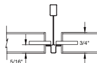
WOODWORKS Square Tegular for INTERLUDE XL HRC Molding F
