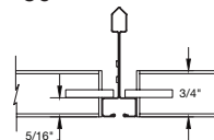
WOODWORKS® Square Tegular for SILHOUETTE® 1/8" Reveal Molding F
