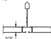
METALWORKS™ 5/16" Square Tegular for SILHOUETTE® 1/8" Reveal Molding E
