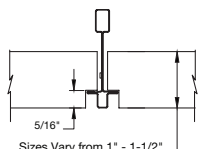
Square Tegular for 9/16" INTERLUDE® Molding F
