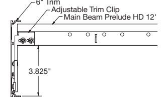
Adjustable Trim Clip (7239) in inverted position
