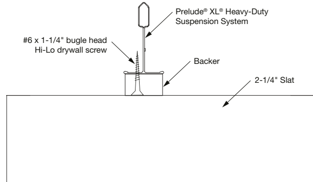
Screw Attachment Detail
