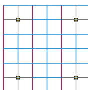
2' × 2' Ceiling layout with lights 8' apart
