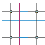
2' × 2' Ceiling layout with lights 6' apart
