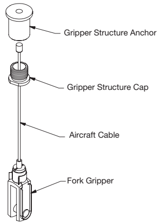
Blades Hanging Kit Assembly
