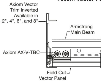
③ Cut Vector Panel with Inverted Axiom Perimeter Trim
