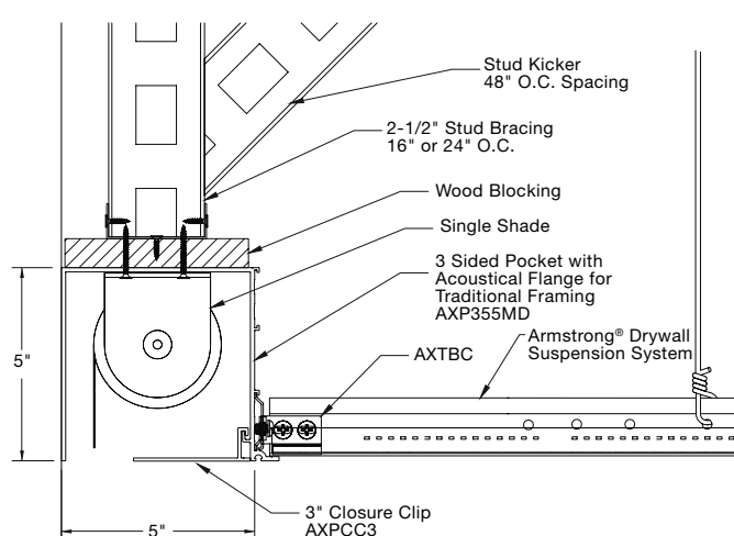
Manual Shade Pocket – For Traditional Framing AXP355MD
