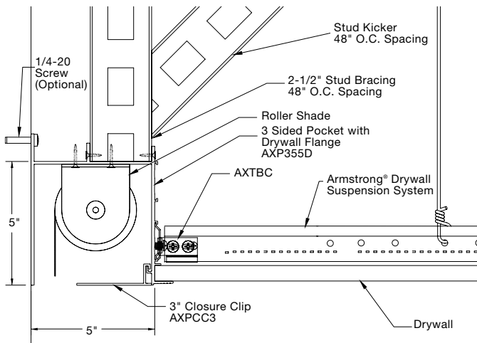
Manual Shade Pocket – For Attachment with 2-1/2" Studs AXP355D
