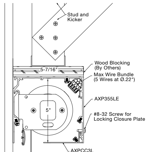
Motorized Shade Pocket – For Traditional Framing AXP355LE
