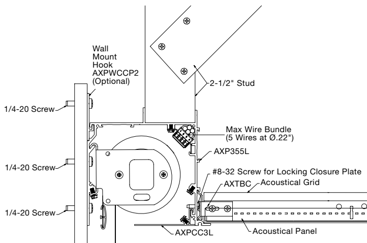
Motorized Shade Pocket – For Attachment with 2-1/2" Studs AXP355L
