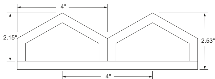
Zenith panel with crowns spaced 4" apart
