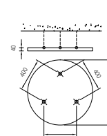
Small Circle Ø 800 x 40 mm
