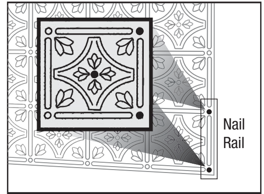
Illustration F Cone Head Nail Placement
