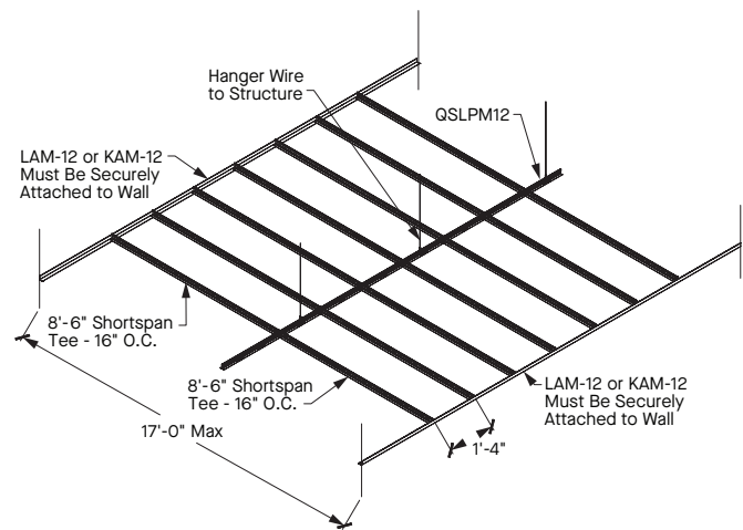
16" O.C. spacing of ShortSpan showing Locking Pocket Mains
