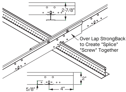
ShortSpan with StrongBack Splice Application
