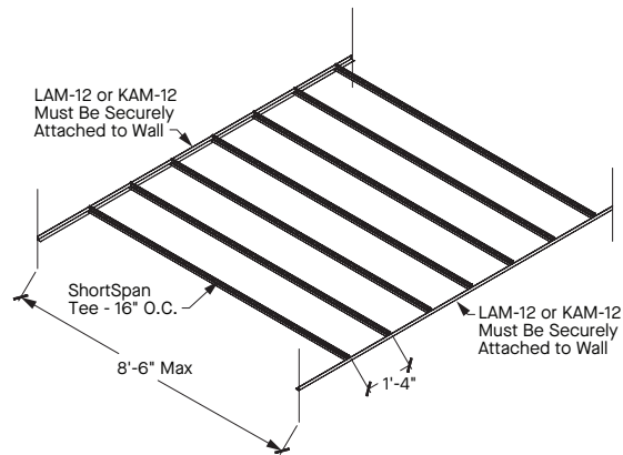
16" O.C. StrongBack at max span of 8'-6"
