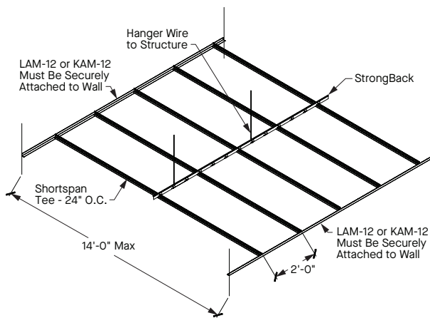
24" O.C. spacing of ShortSpan® showing StrongBack™
