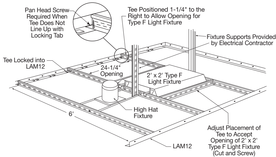
Fixture Installation
