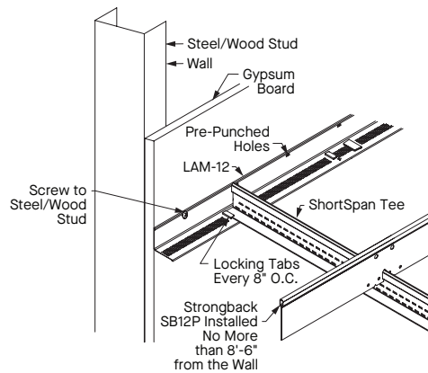
ShortSpan at Wall
