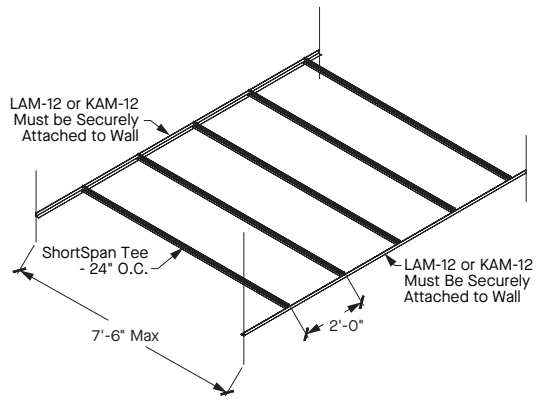
24" O.C. spacing of ShortSpan at max span of 7'-6"
