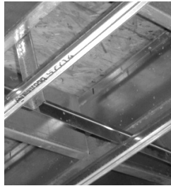
Manufactured StrongBack
