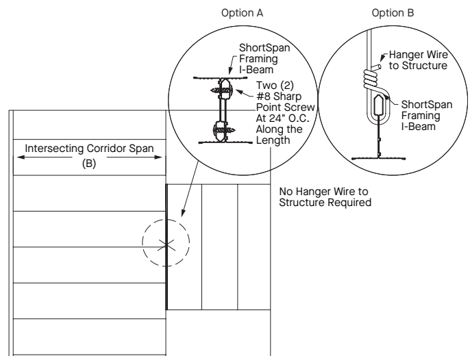
ShortSpan Intersection Corridors with I-Beam Girder
