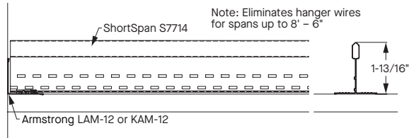
ShortSpan at Perimeter Wall
