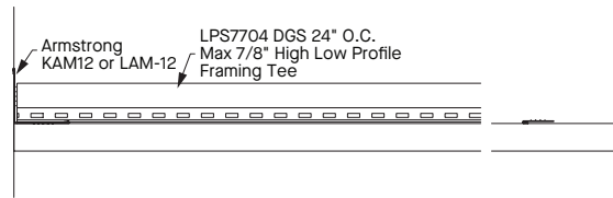
ShortSpan Low Profile at Perimeter Wall
